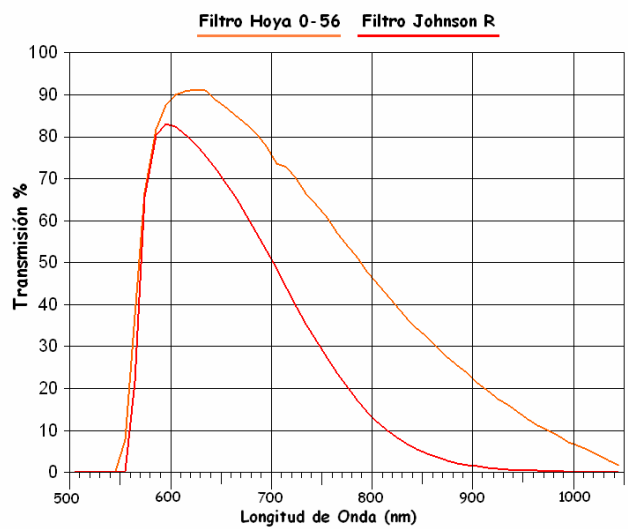
R Johnson CCD SONY ICX429ALL-7
